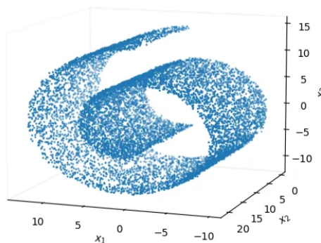
Figura 13: Swiss roll [14].
